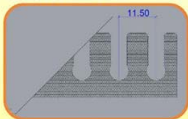
Passo 11.5 - Pitch 11.5
