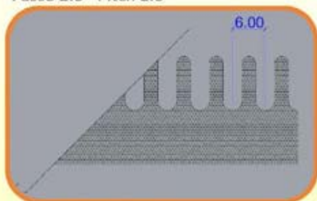
Passo 6.0 - Pitch 6.0
